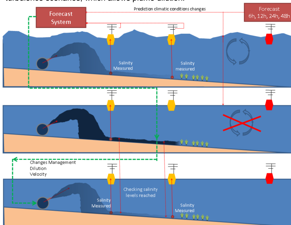
Figure 5.- Conceptual outline of the Adaptive Management operation in forecasting climatic changes.
