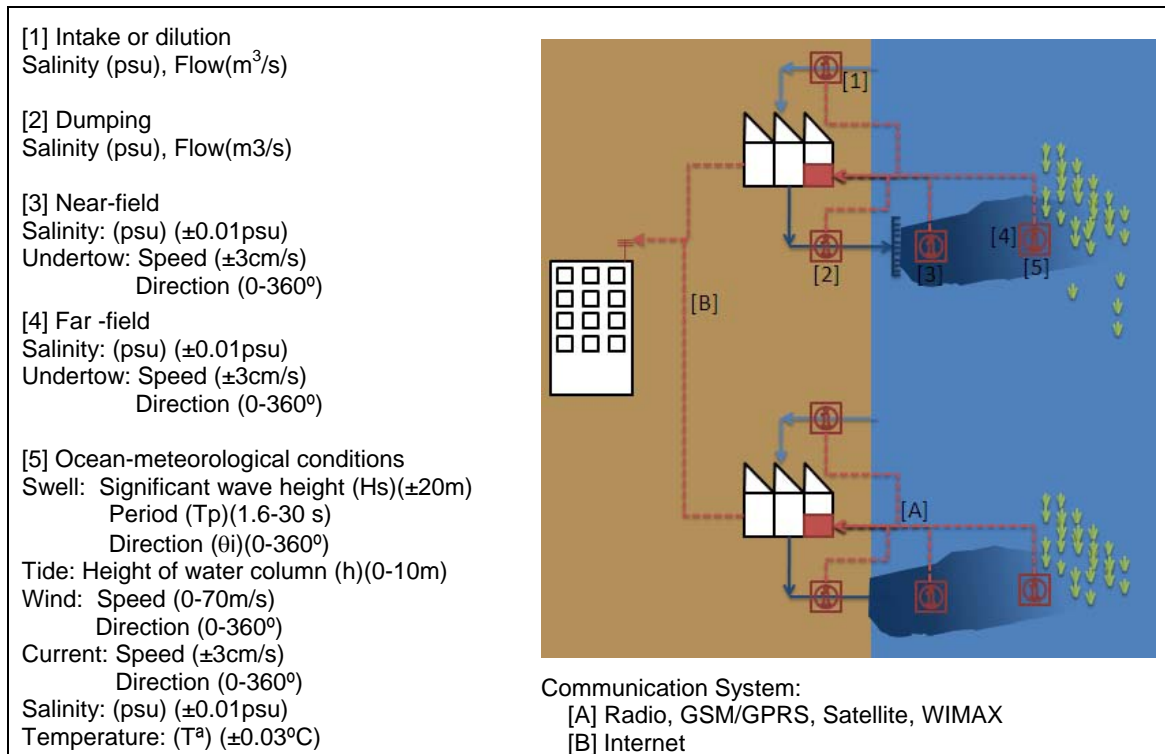
Figure 1.- Outline of the implementation of sensors and communications.
