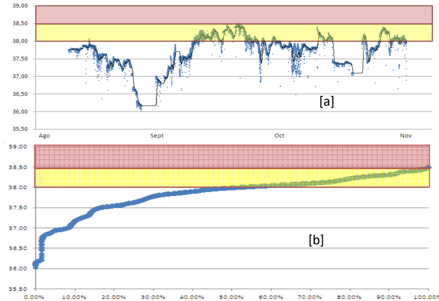
Figure 2.- Evolution of observed salinity (psu) every 5min at a depth of 20cm in a monitoring CTD of a brine dump and alarm levels [a]. Non-exceedance percentile during the time of the observations in September [b].
